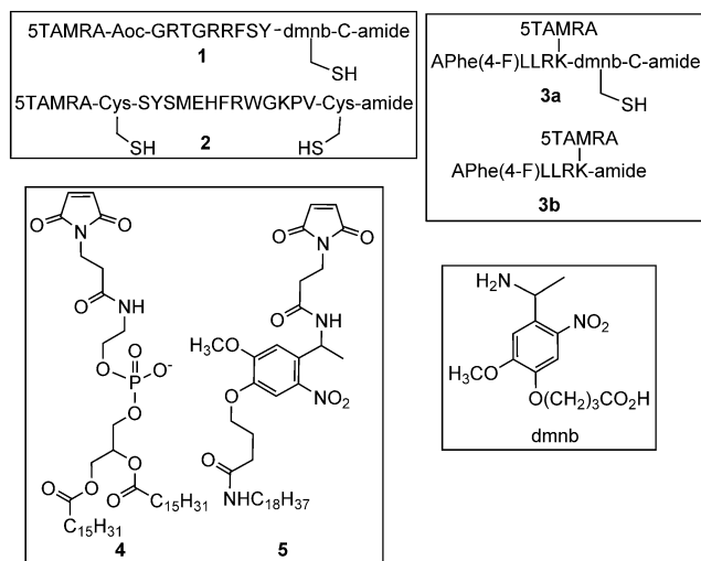
Scheme 1. Structures of the peptide (1–3) and linker/lipid anchor (4,5) modules used in this study, along with the photocleavable unit dmnb.
